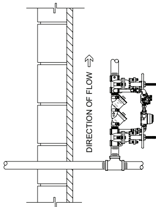
VERTICAL INSTALLATION
