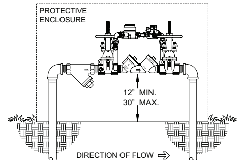
OUTDOOR INSTALLATION
