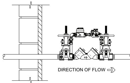
INDOOR INSTALLATION
