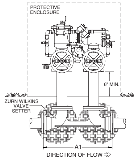
OUTDOOR INSTALLATION
