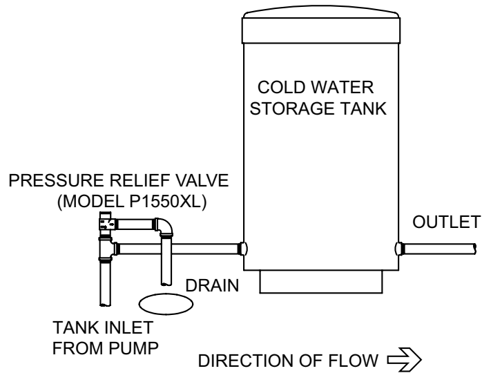
TYPICAL INSTALLATION (PUMP PRESSURE RELIEF)
