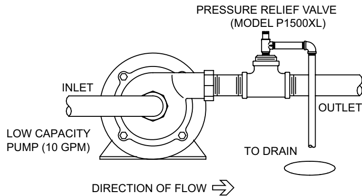
TYPICAL INSTALLATION (PUMP PRESSURE RELIEF)
